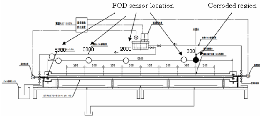
Fig 5 Experimental mock-up
